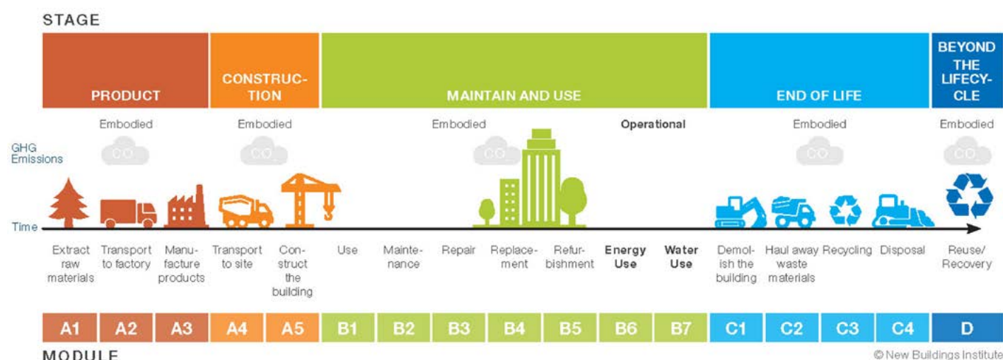
Figure 19: Lifecycle Stages of Buildings and Whole-Life Carbon Emissions 128
