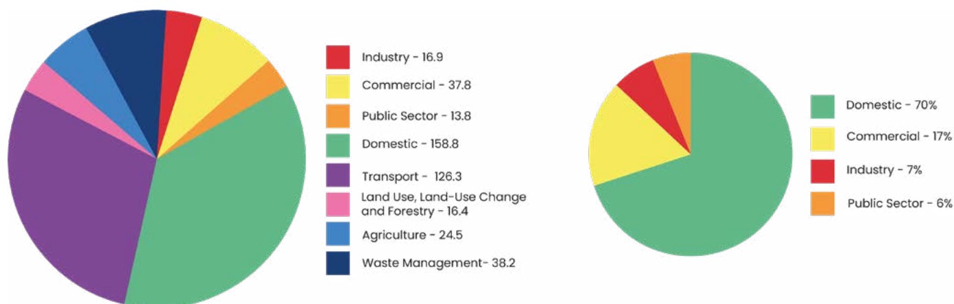
Figure 21: 2022 Total Area-wide Emissions in East Dunbartonshire (kt CO 2 e) by Sector (left) and Emission Percentage from Built Sectors (right)
