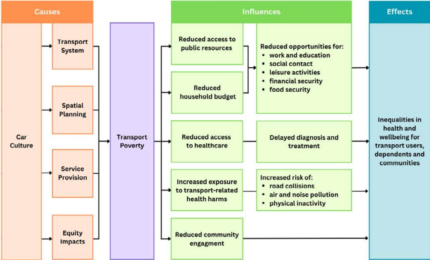
Figure 17: A model of transport poverty – the causes and influences on health and health inequalities (adapted figure from Public Health Scotland) 101
